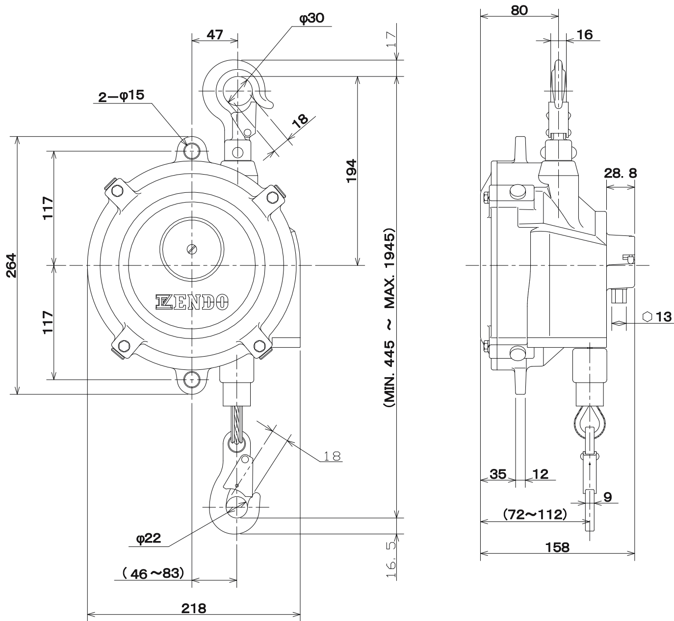
SPRING BALANCER EWF-30
